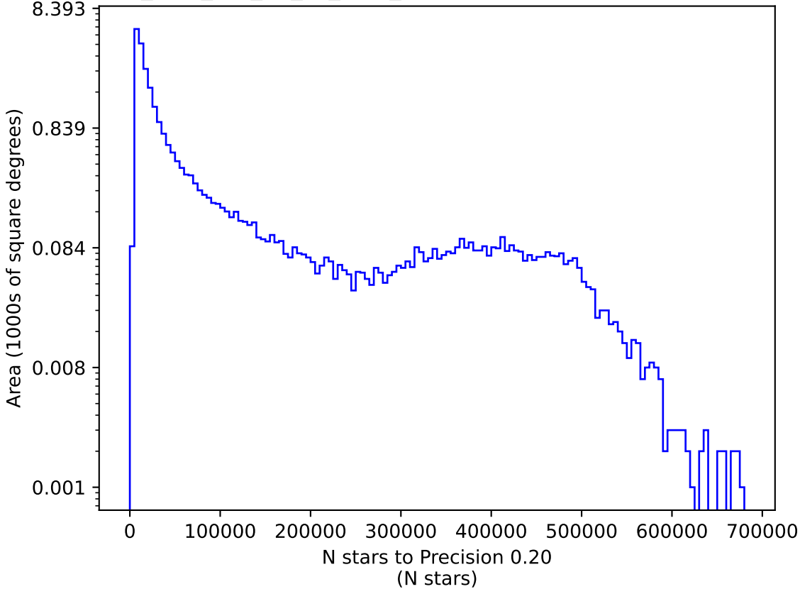
too_elab_r64_d2_gz_v3.4_10yrs i: N stars to Precision 0.20
