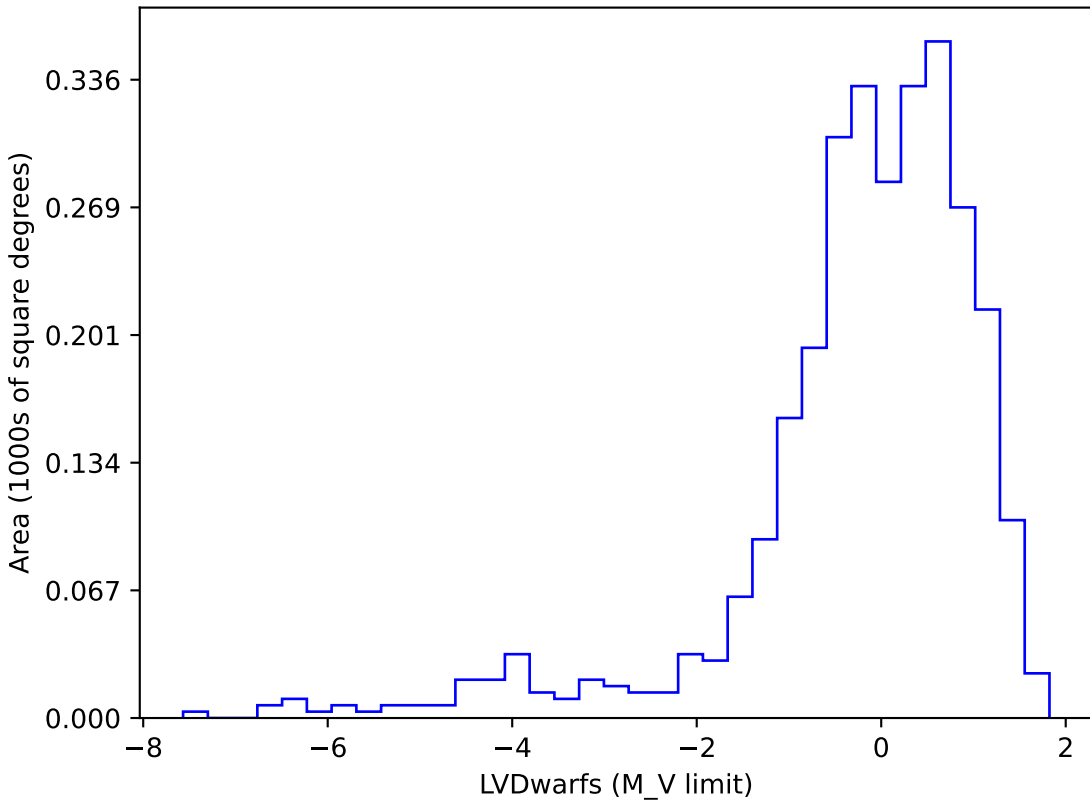
too_elab_r64_d2_gz_v3.4_10yrs gi SCP: LVDwarfs
