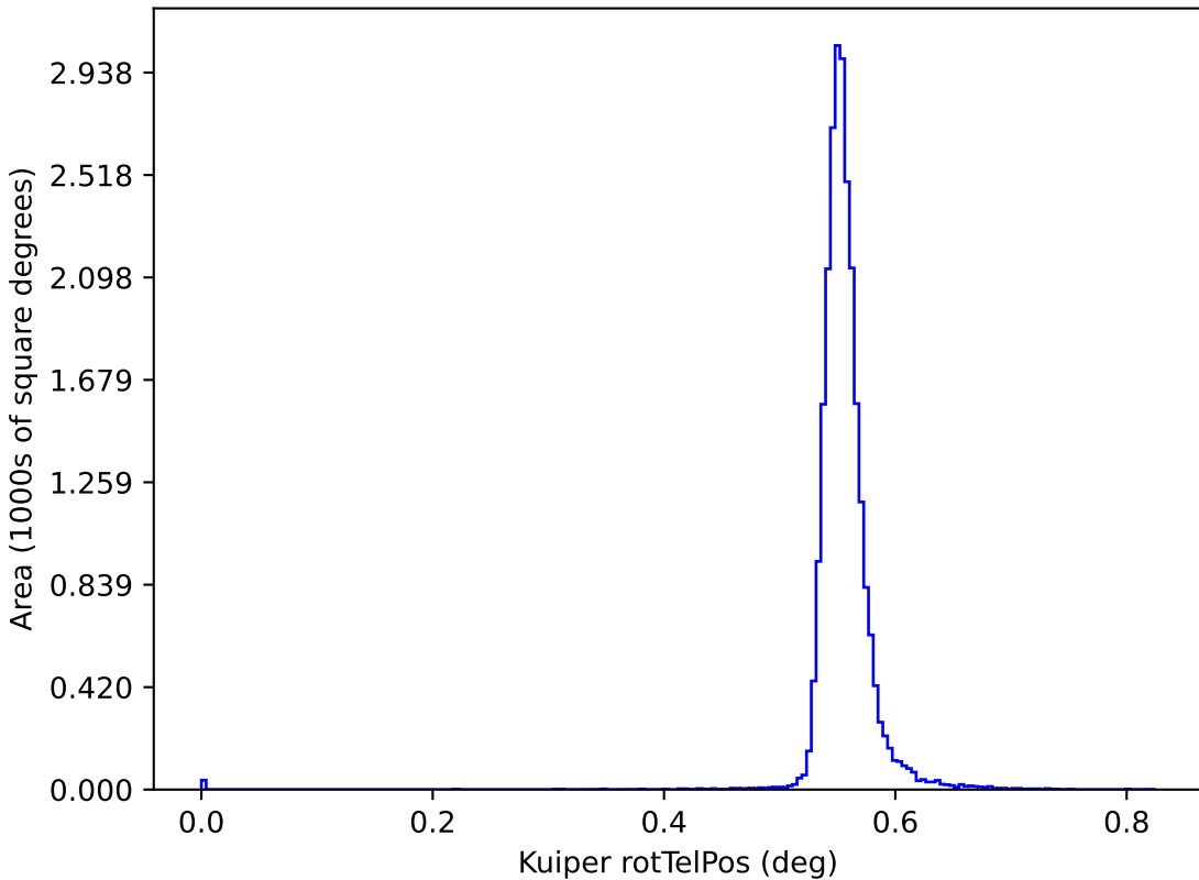
too_elab_r64_d2_gz_v3.4_10yrs y: Kuiper rotTelPos
