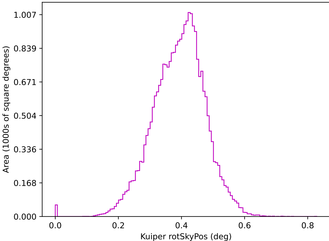
too_elab_r64_d2_gz_v3.4_10yrs z: Kuiper rotSkyPos
