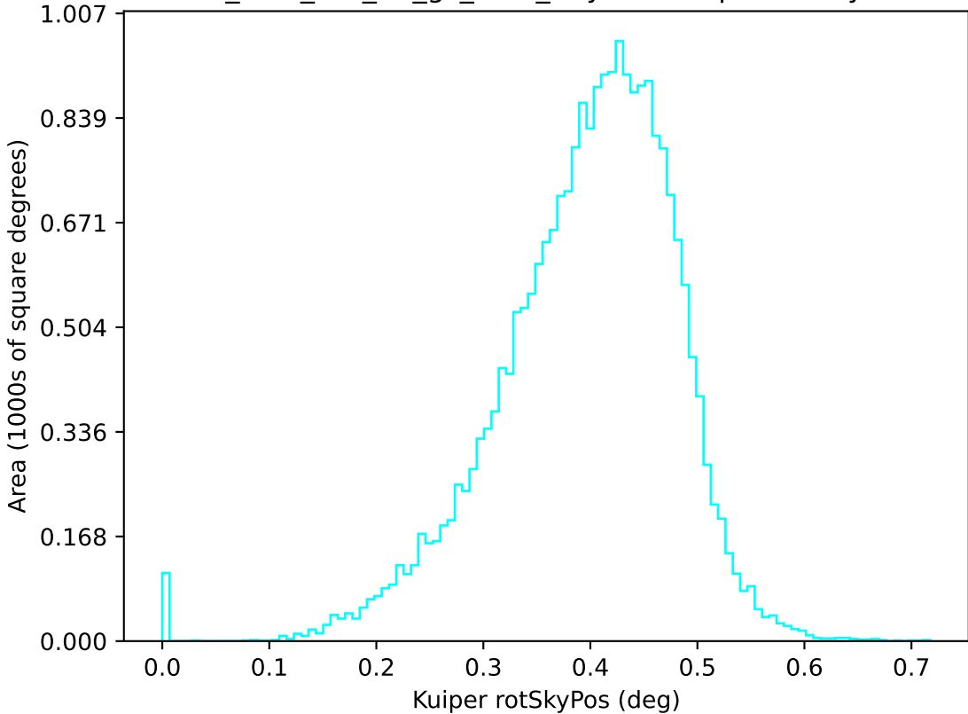
too_elab_r64_d2_gz_v3.4_10yrs u: Kuiper rotSkyPos
