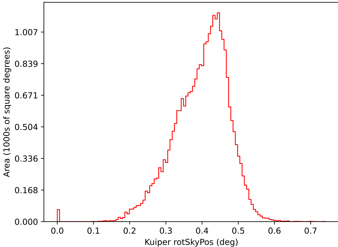
too_elab_r64_d2_gz_v3.4_10yrs i: Kuiper rotSkyPos
