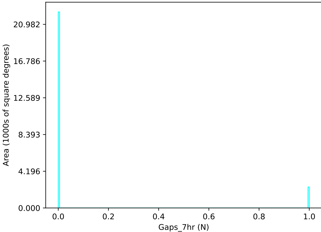
too_elab_r64_d2_gz_v3.4_10yrs u band: Gaps_7hr
