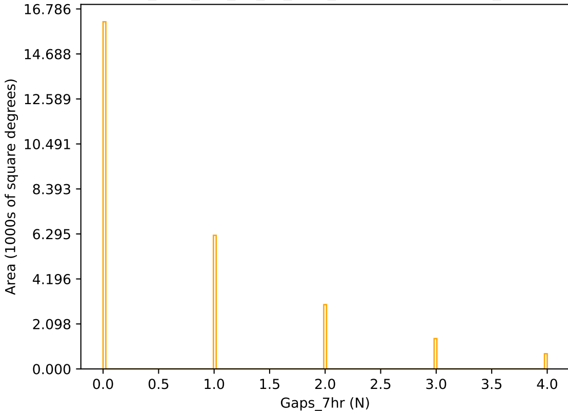
too_elab_r64_d2_gz_v3.4_10yrs r band: Gaps_7hr
