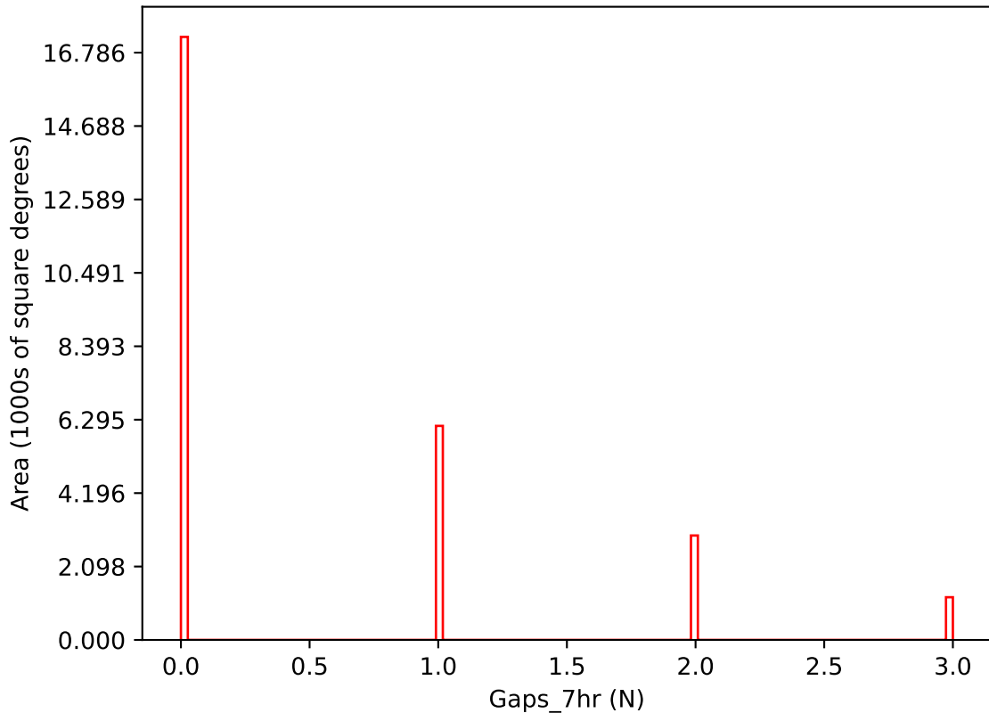
too_elab_r64_d2_gz_v3.4_10yrs i band: Gaps_7hr
