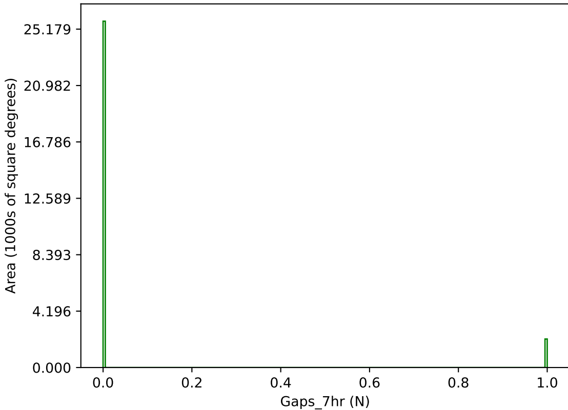
too_elab_r64_d2_gz_v3.4_10yrs g band: Gaps_7hr
