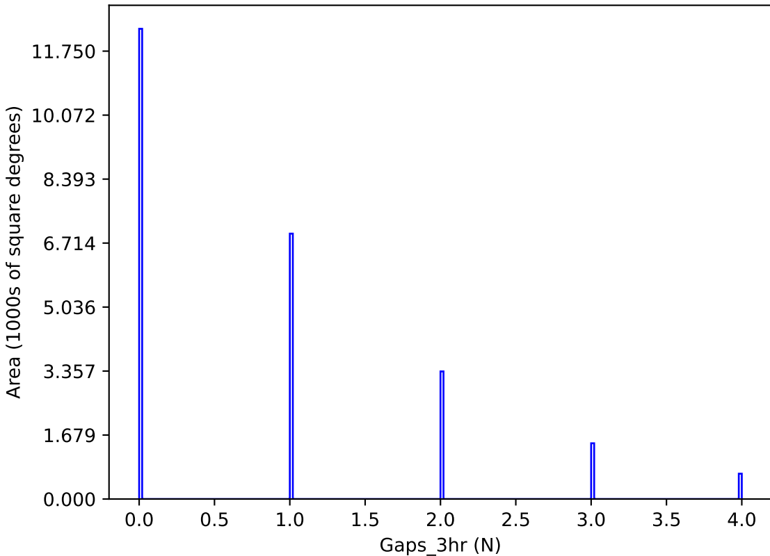
too_elab_r64_d2_gz_v3.4_10yrs y band: Gaps_3hr
