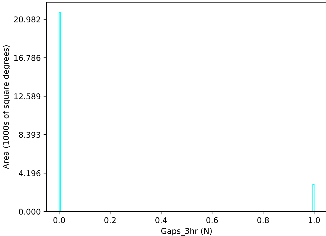
too_elab_r64_d2_gz_v3.4_10yrs u band: Gaps_3hr
