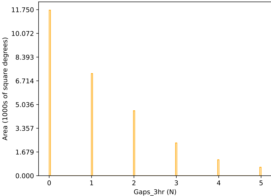
too_elab_r64_d2_gz_v3.4_10yrs r band: Gaps_3hr
