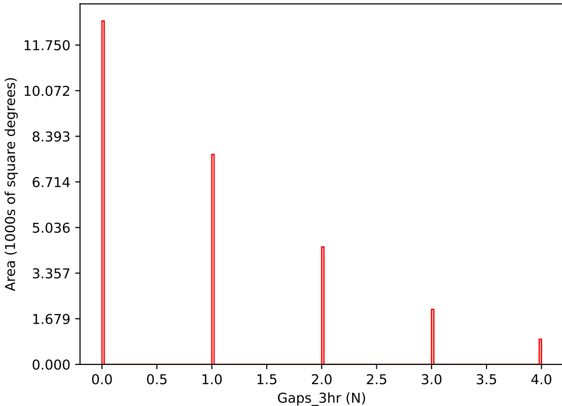
too_elab_r64_d2_gz_v3.4_10yrs i band: Gaps_3hr
