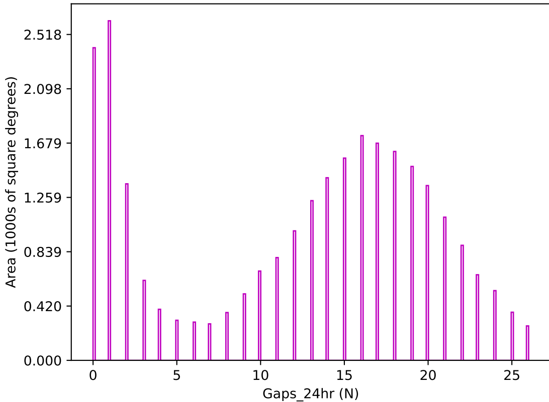
too_elab_r64_d2_gz_v3.4_10yrs z band: Gaps_24hr
