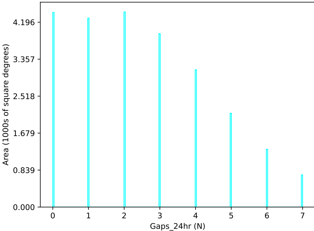
too_elab_r64_d2_gz_v3.4_10yrs u band: Gaps_24hr
