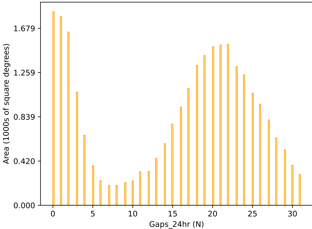
too_elab_r64_d2_gz_v3.4_10yrs r band: Gaps_24hr
