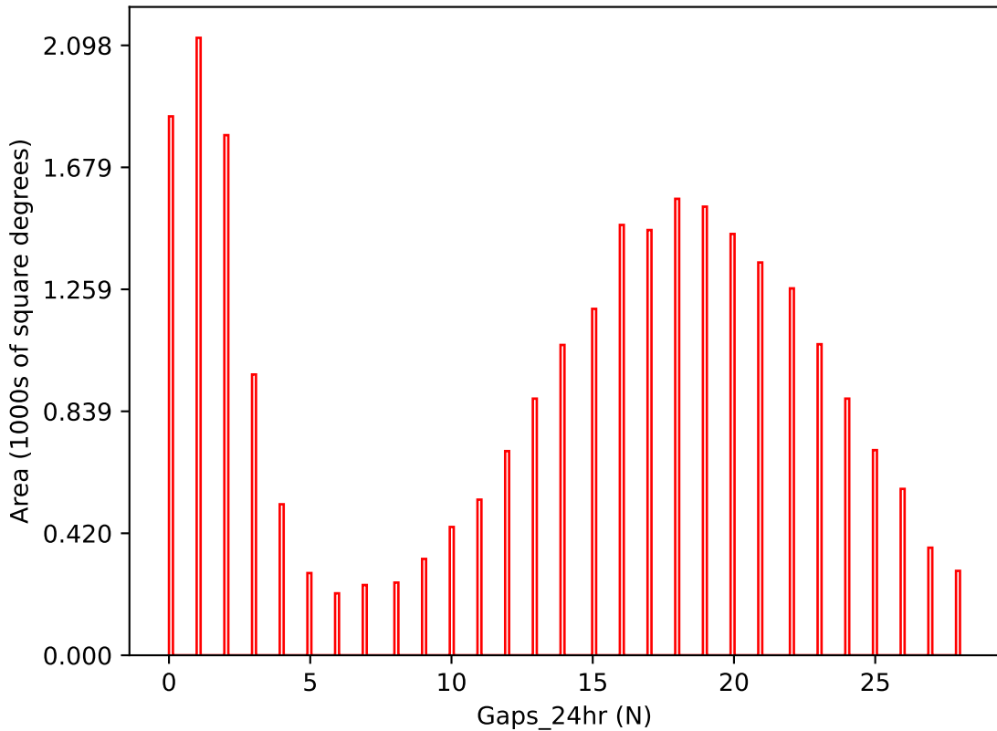
too_elab_r64_d2_gz_v3.4_10yrs i band: Gaps_24hr
