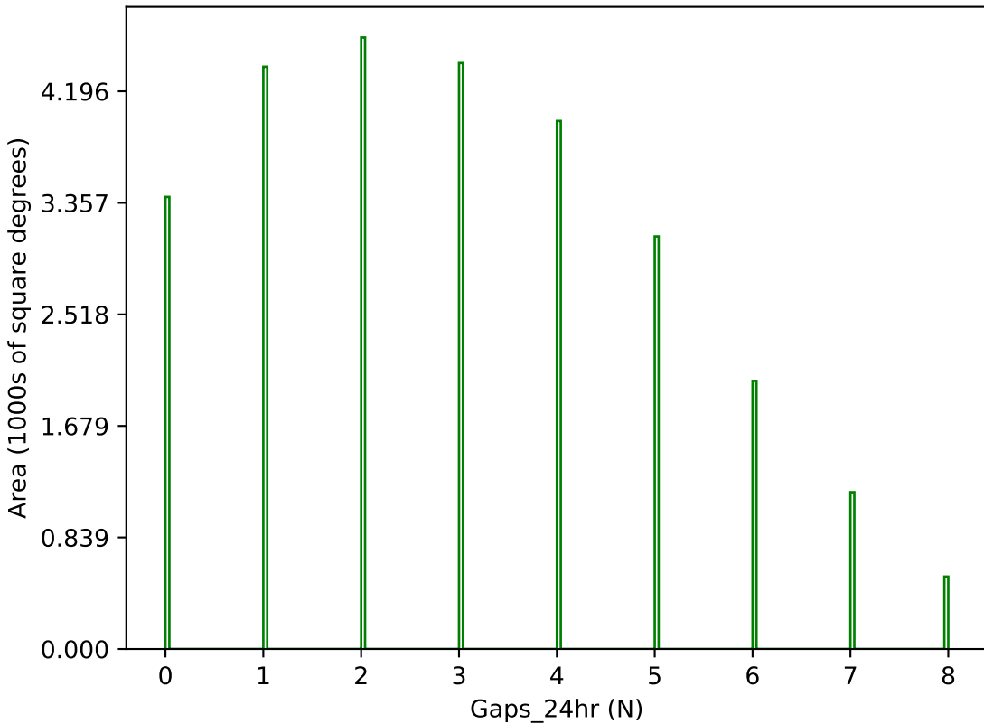
too_elab_r64_d2_gz_v3.4_10yrs g band: Gaps_24hr
