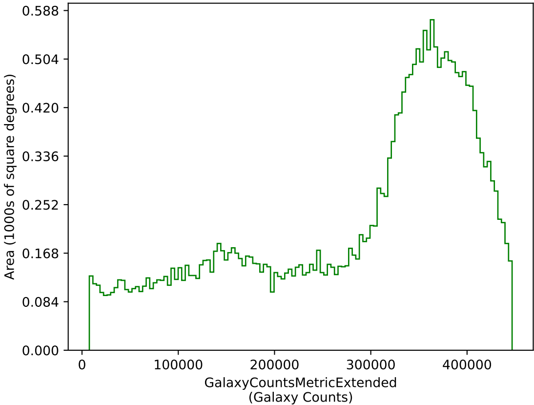
too_elab_r64_d2_gz_v3.4_10yrs g: GalaxyCountsMetricExtended
