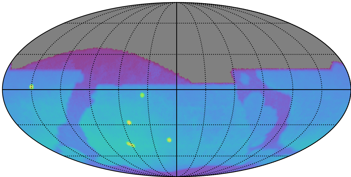
too_elab_r64_d2_gz_v3.4_10yrs : Brown Dwarf, L7
