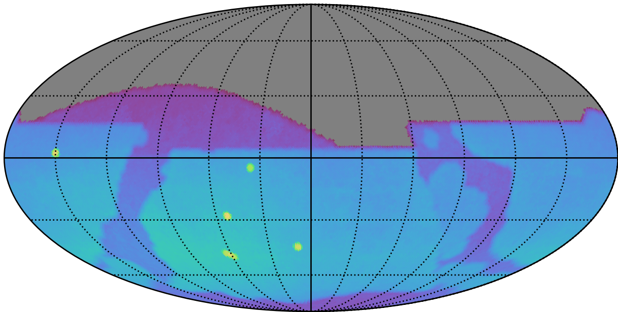
too_elab_r64_d2_gz_v3.4_10yrs : Brown Dwarf, L4
