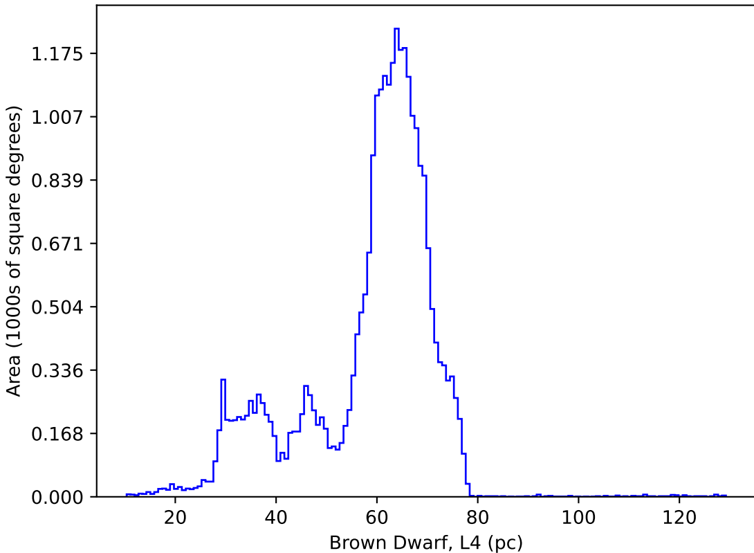
too_elab_r64_d2_gz_v3.4_10yrs : Brown Dwarf, L4
