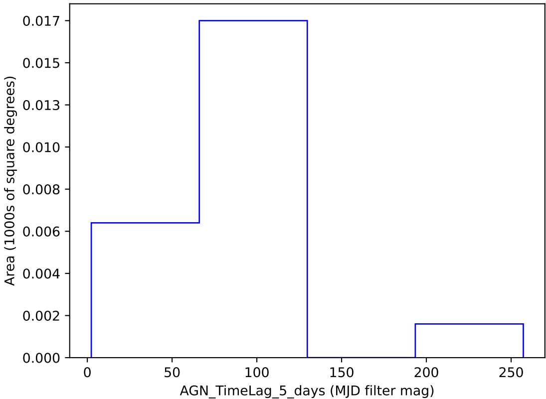
too_elab_r64_d2_gz_v3.4_10yrs y band: AGN_TimeLag_5_days
