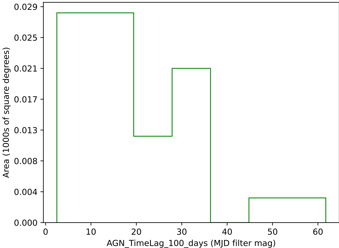
too_elab_r64_d2_gz_v3.4_10yrs g band: AGN_TimeLag_100_days
