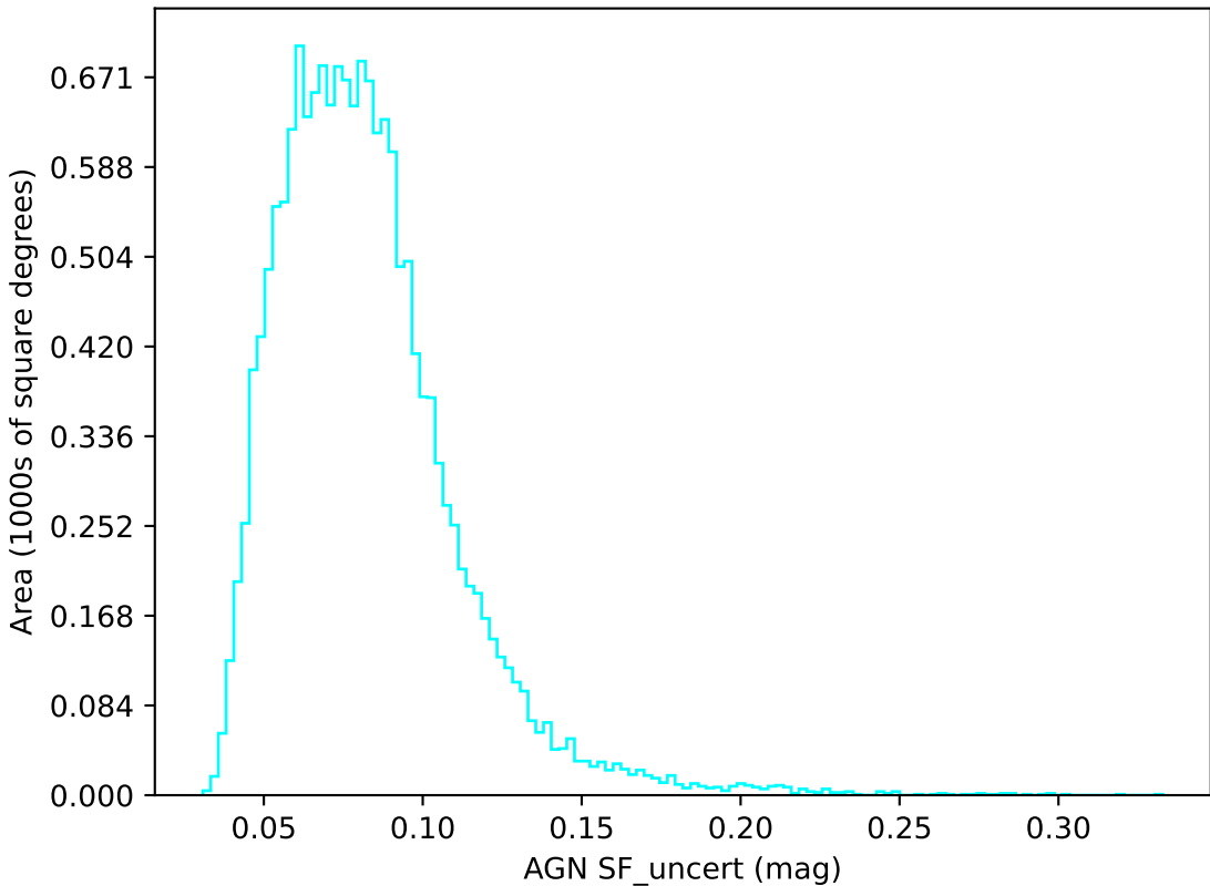
too_elab_r64_d2_gz_v3.4_10yrs u band: AGN SF_uncert
