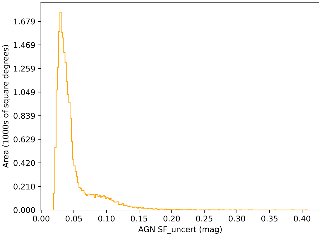
too_elab_r64_d2_gz_v3.4_10yrs r band: AGN SF_uncert
