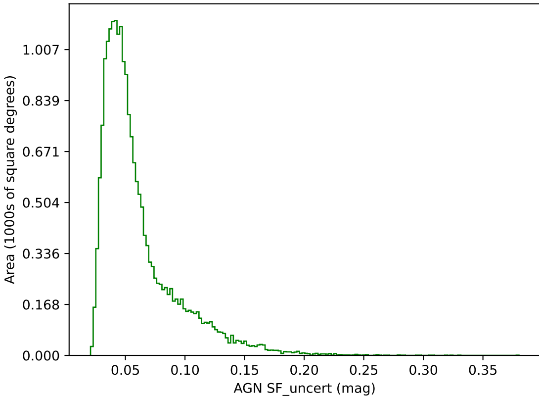
too_elab_r64_d2_gz_v3.4_10yrs g band: AGN SF_uncert
