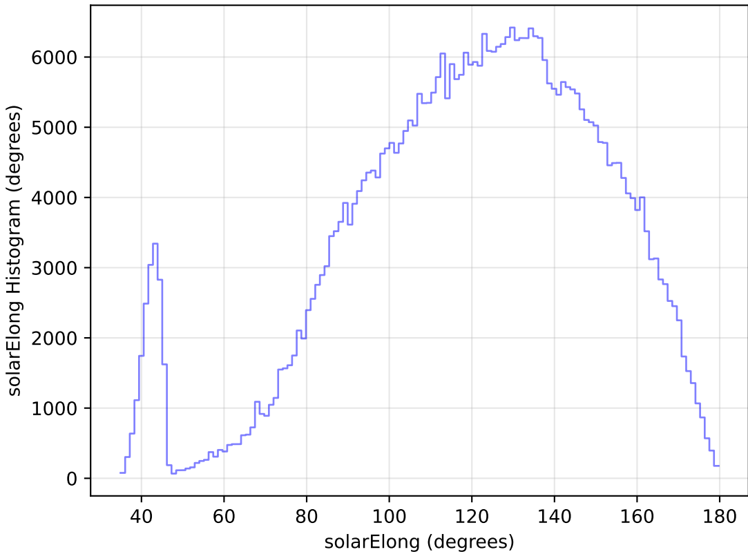
too_elab_r64_d2_gz_v3.4_10yrs WFD z band: solarElong Histogram
