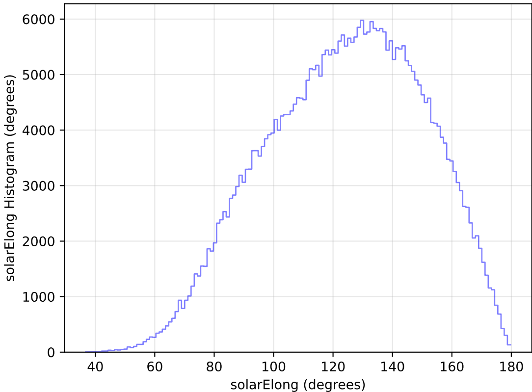
too_elab_r64_d2_gz_v3.4_10yrs WFD y band: solarElong Histogram
