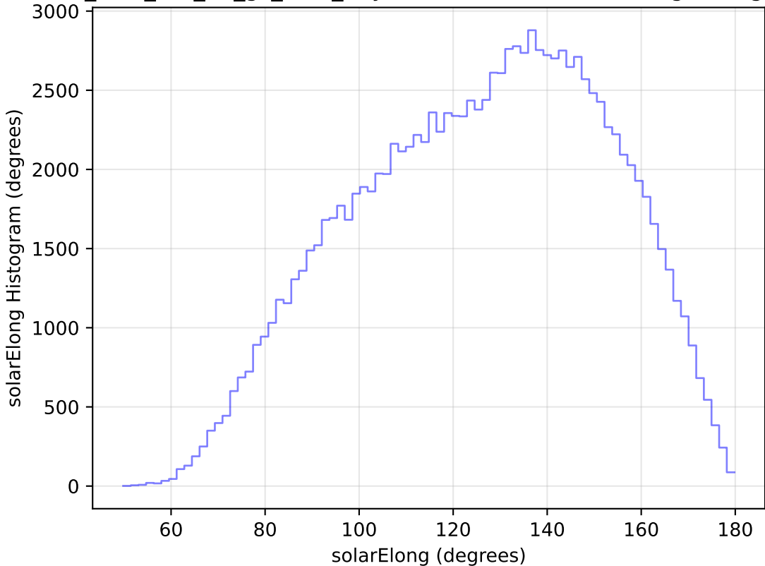
too_elab_r64_d2_gz_v3.4_10yrs WFD u band: solarElong Histogram
