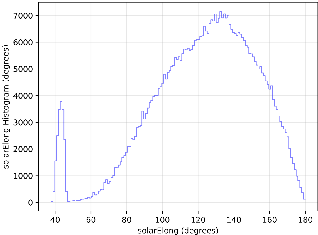
too_elab_r64_d2_gz_v3.4_10yrs WFD r band: solarElong Histogram
