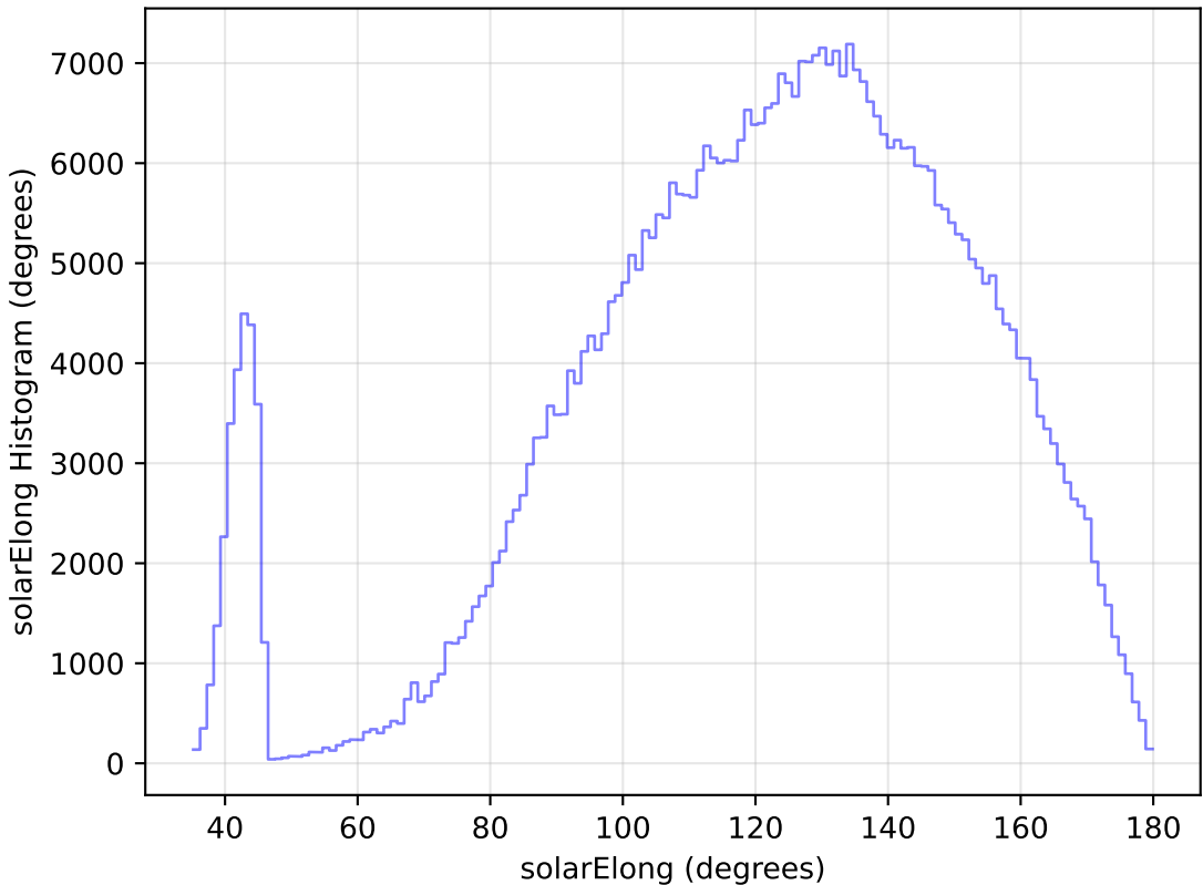
too_elab_r64_d2_gz_v3.4_10yrs WFD i band: solarElong Histogram
