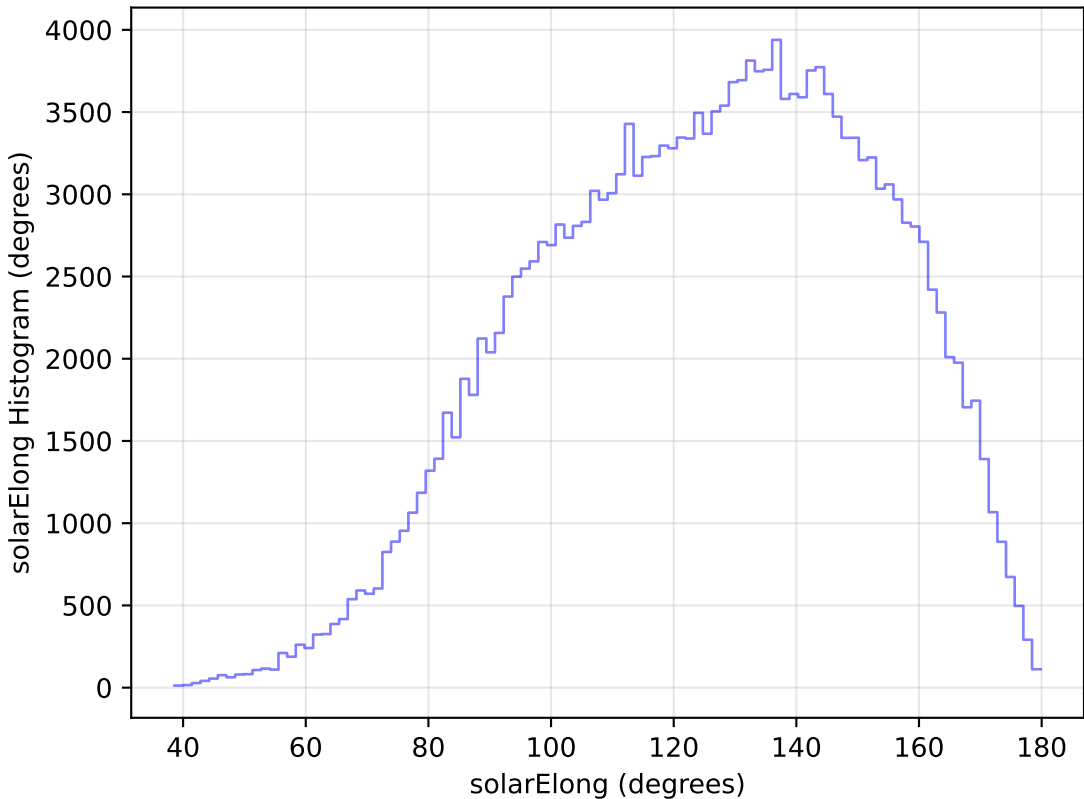
too_elab_r64_d2_gz_v3.4_10yrs WFD g band: solarElong Histogram
