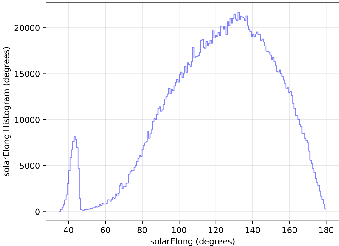
too_elab_r64_d2_gz_v3.4_10yrs WFD all bands: solarElong Histogram
