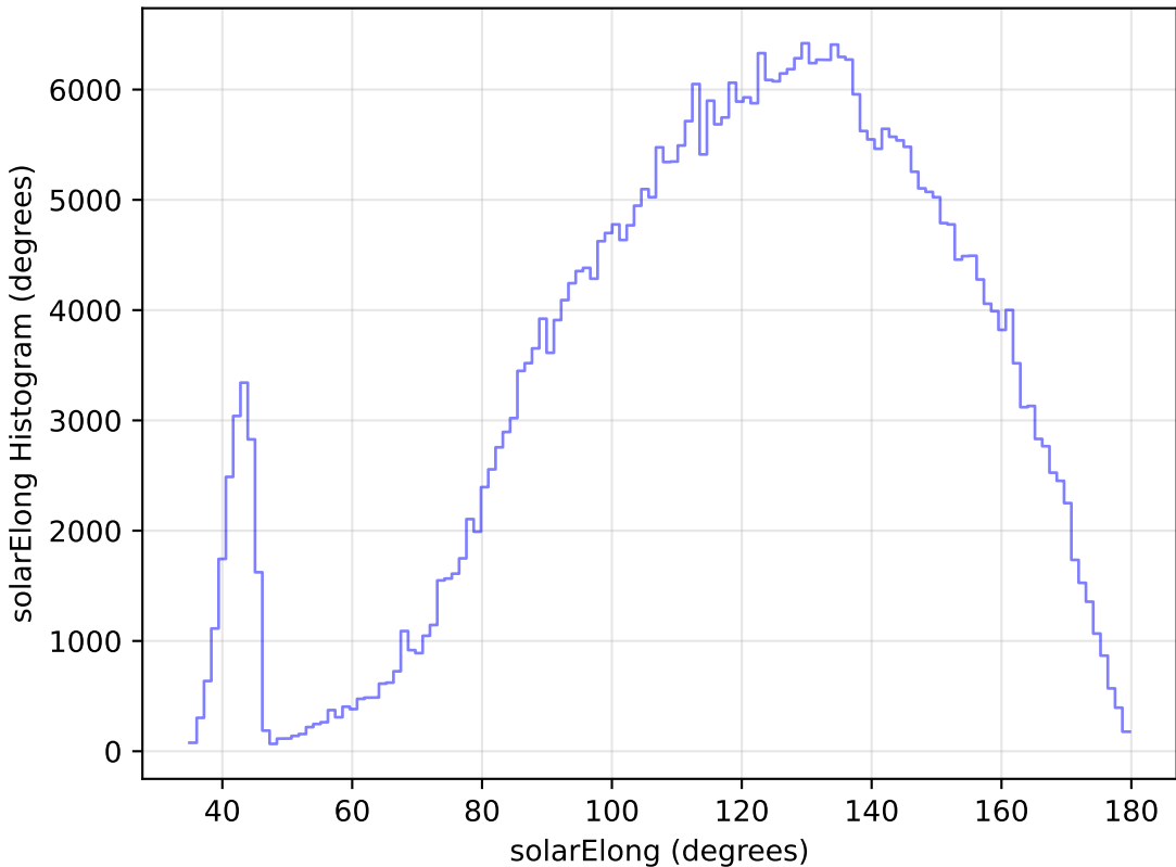
too_elab_r64_d2_gz_v3.4_10yrs All sky z band: solarElong Histogram
