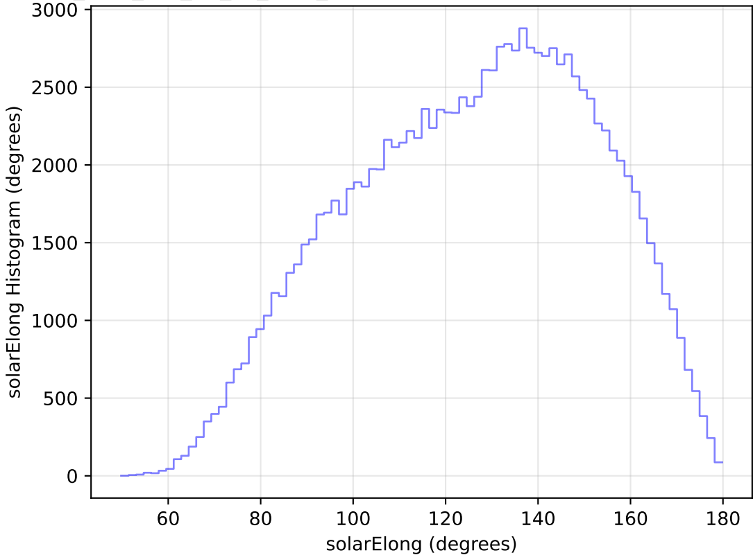
too_elab_r64_d2_gz_v3.4_10yrs All sky u band: solarElong Histogram
