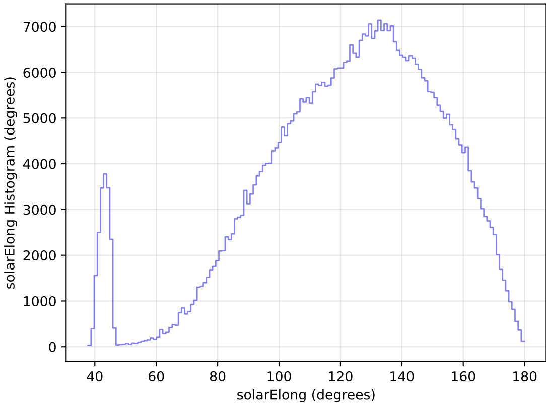
too_elab_r64_d2_gz_v3.4_10yrs All sky r band: solarElong Histogram
