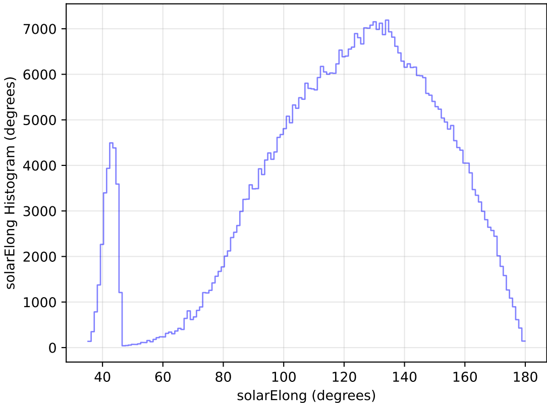
too_elab_r64_d2_gz_v3.4_10yrs All sky i band: solarElong Histogram
