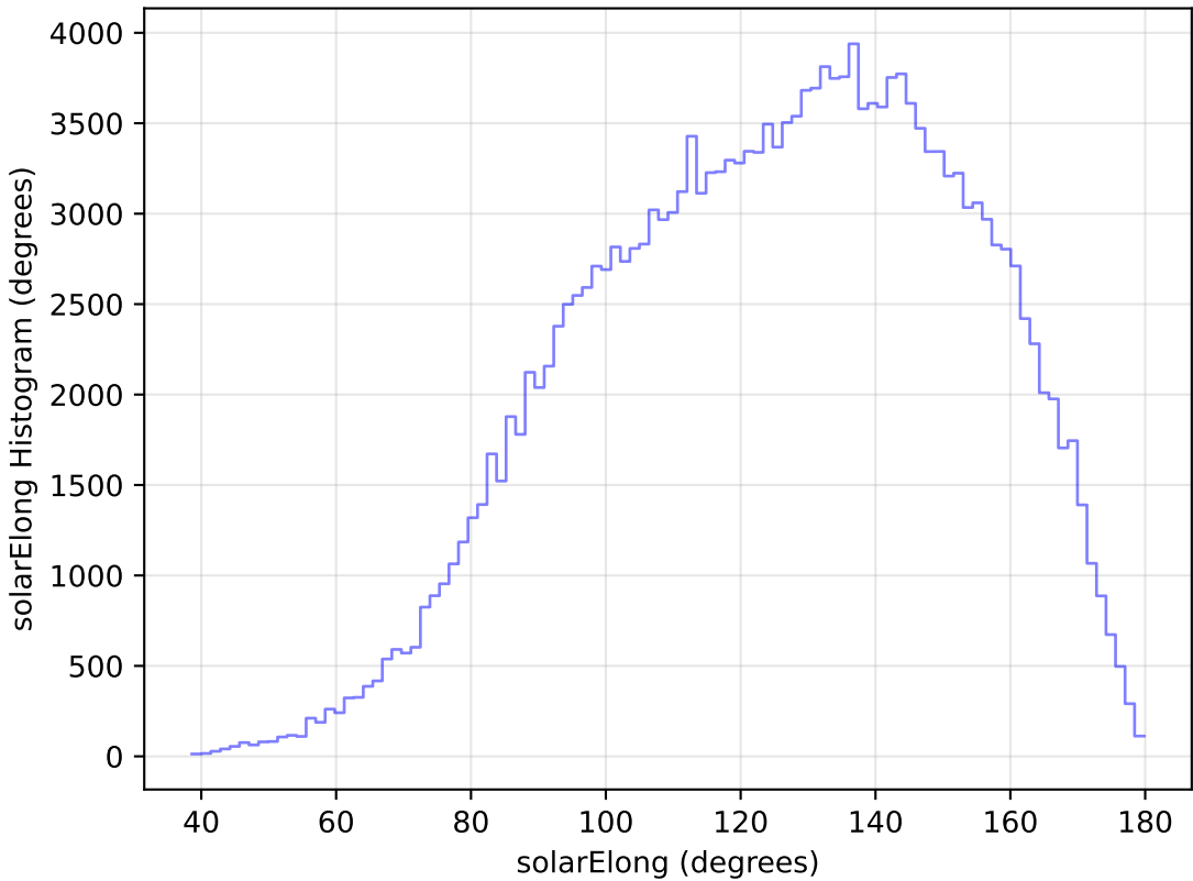
too_elab_r64_d2_gz_v3.4_10yrs All sky g band: solarElong Histogram
