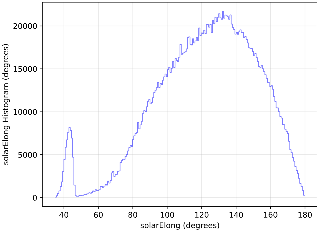
too_elab_r64_d2_gz_v3.4_10yrs All sky all bands: solarElong Histogram
