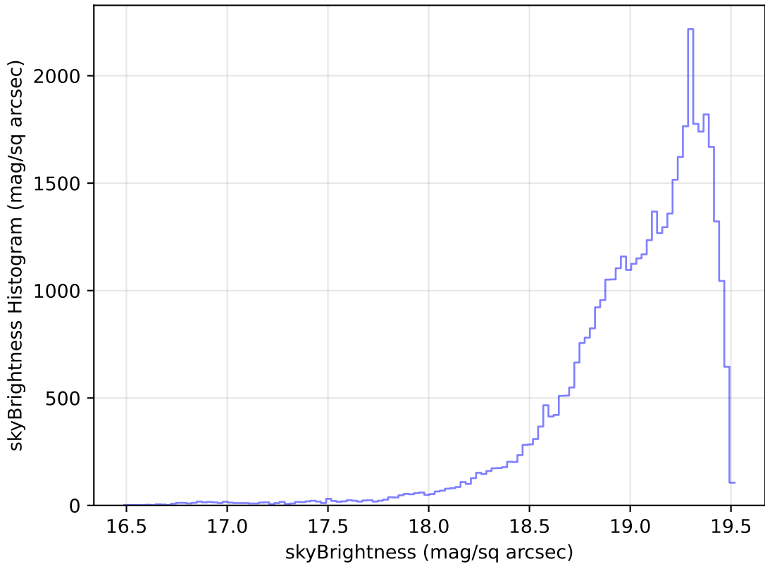
too_elab_r64_d2_gz_v3.4_10yrs Yr 1 z band: skyBrightness Histogram
