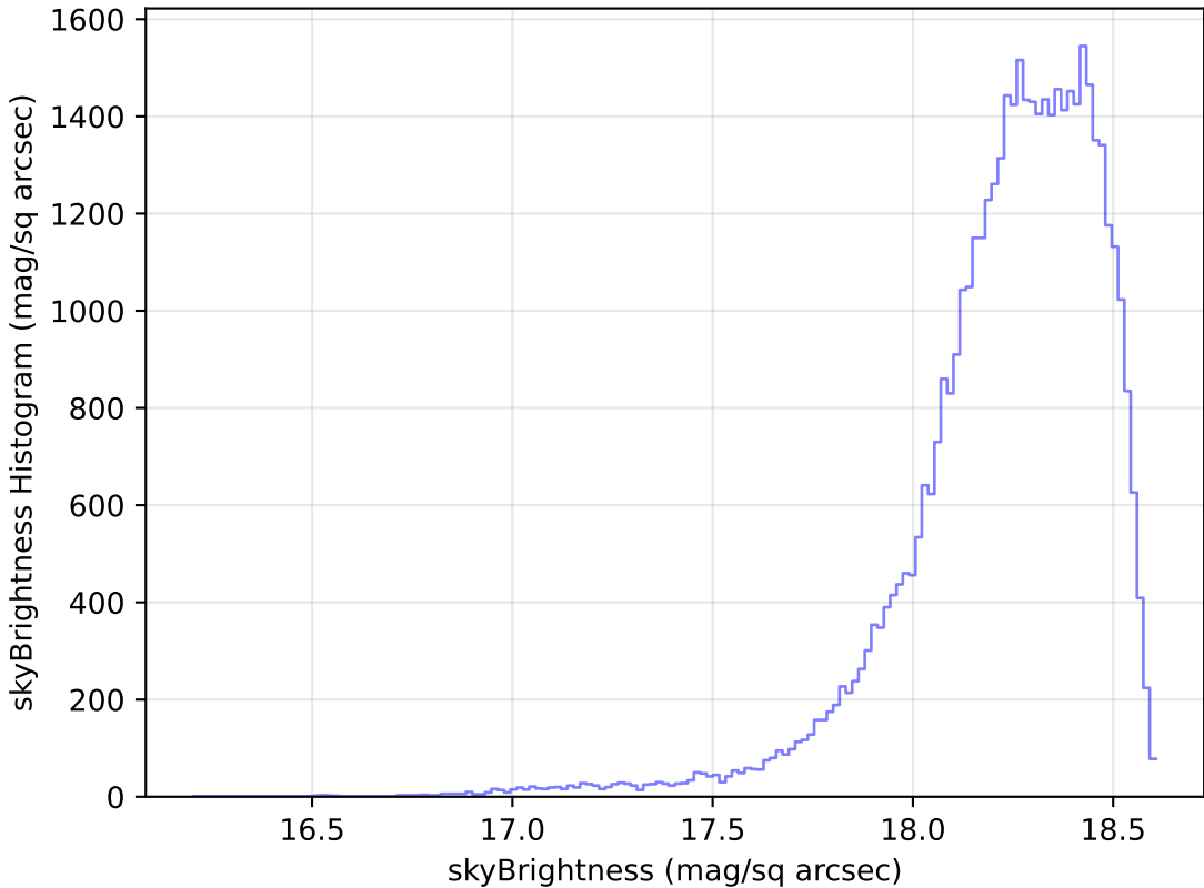
too_elab_r64_d2_gz_v3.4_10yrs Yr 1 y band: skyBrightness Histogram
