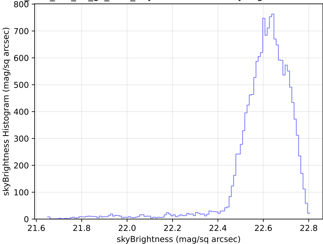
too_elab_r64_d2_gz_v3.4_10yrs Yr 1 u band: skyBrightness Histogram
