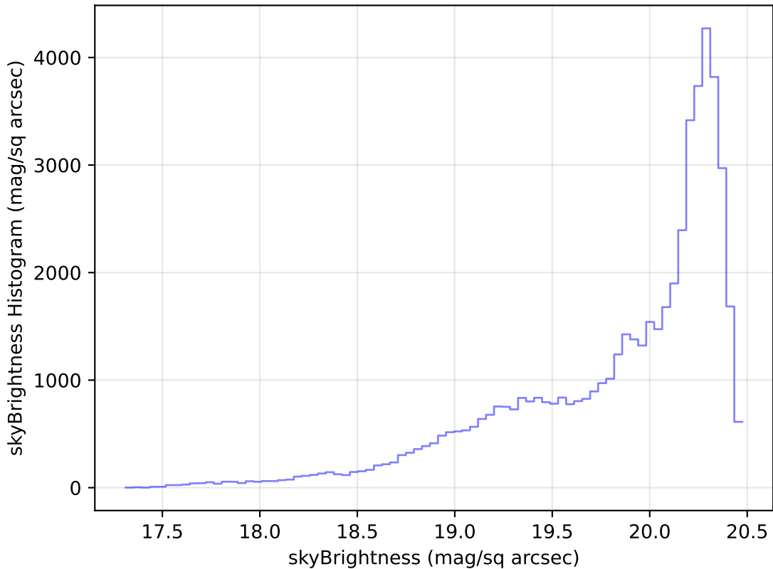
too_elab_r64_d2_gz_v3.4_10yrs Yr 1 i band: skyBrightness Histogram
