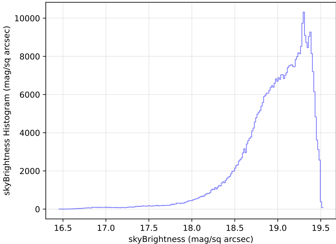
too_elab_r64_d2_gz_v3.4_10yrs WFD z band: skyBrightness Histogram
