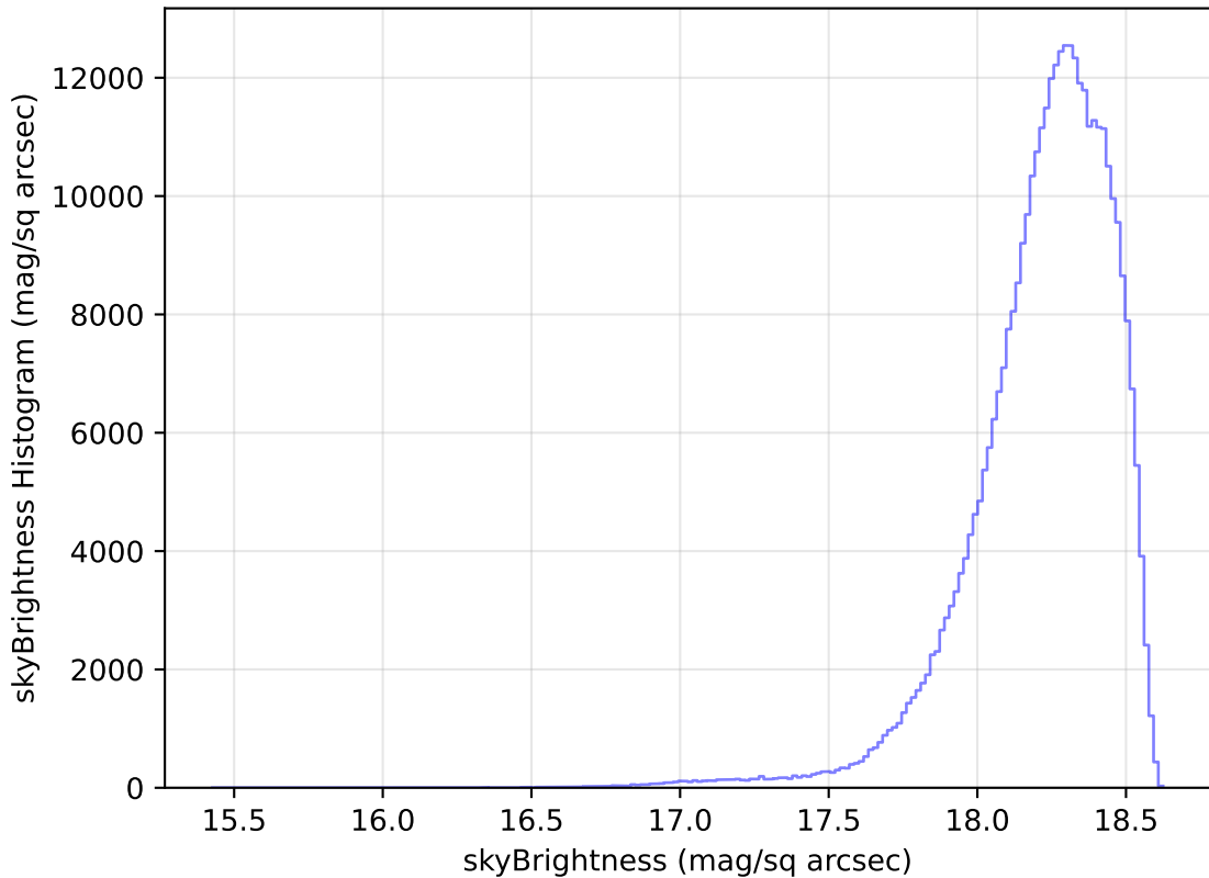
too_elab_r64_d2_gz_v3.4_10yrs WFD y band: skyBrightness Histogram
