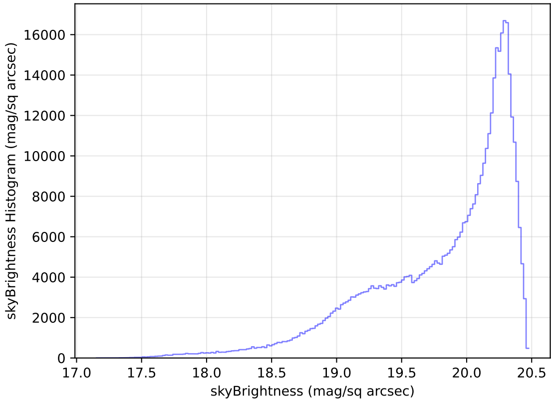
too_elab_r64_d2_gz_v3.4_10yrs WFD i band: skyBrightness Histogram
