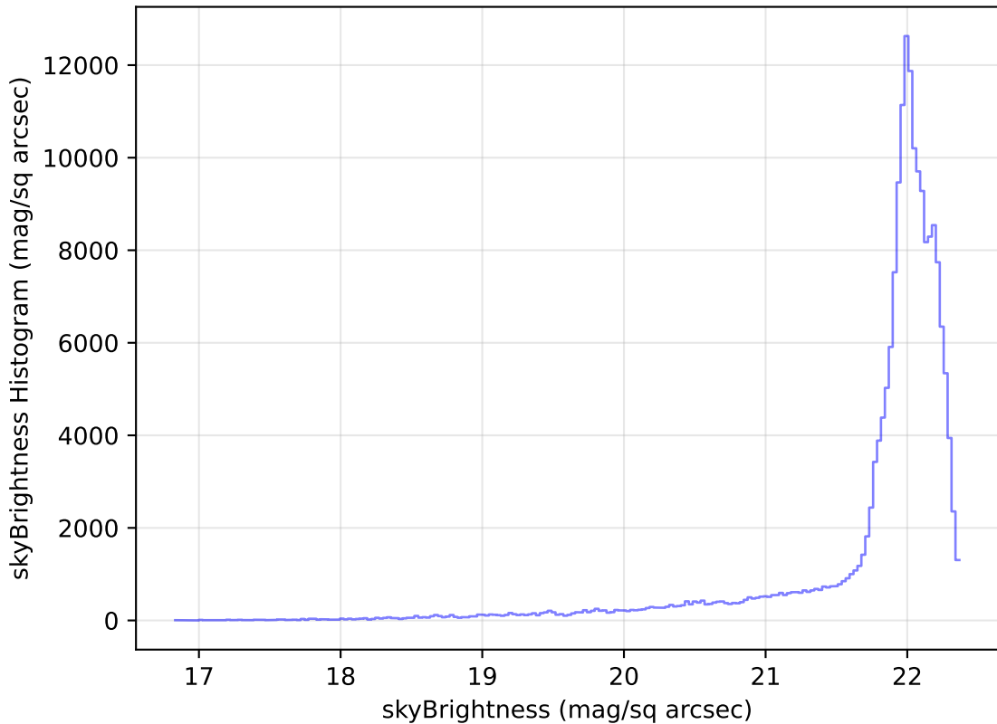
too_elab_r64_d2_gz_v3.4_10yrs WFD g band: skyBrightness Histogram
