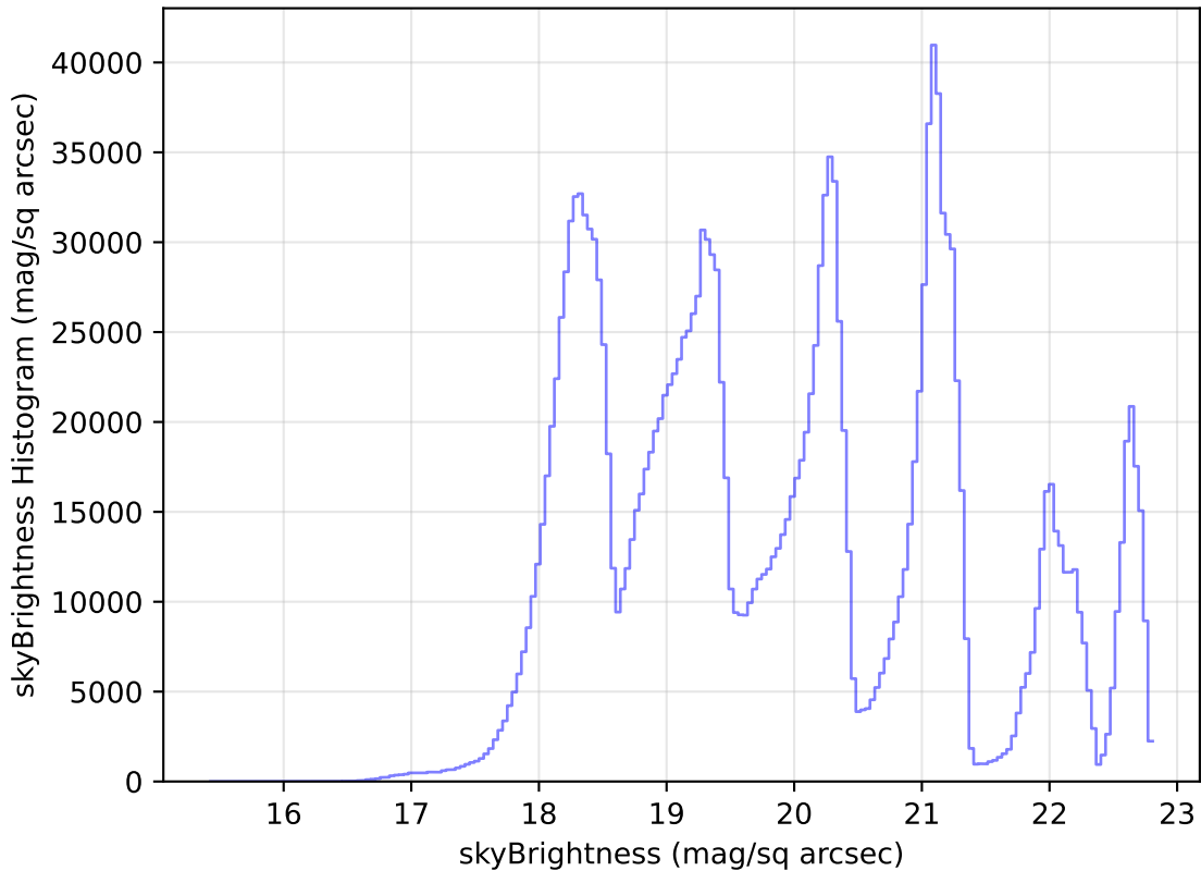
too_elab_r64_d2_gz_v3.4_10yrs WFD all bands: skyBrightness Histogram
